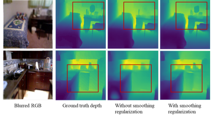
Fig. 4: Results with and without the smoothing regularization for depth estimation on NYU-v2 dataset. The deblurring loss is L_{charb} . The rectangular crops illustrate areas where new details emerge when using smoothing regularization.
