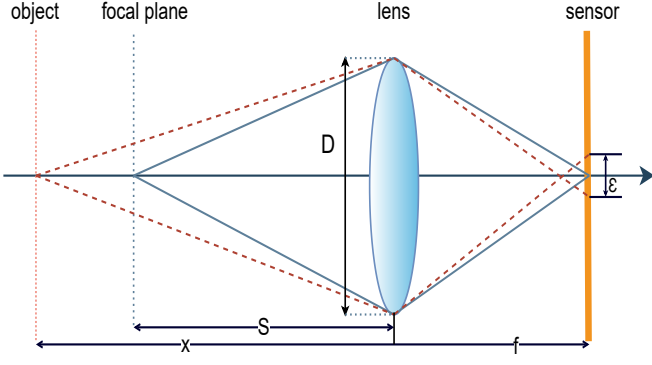
Fig. 3: The thin lens model: the COC diameter \varepsilon depends on the distance x of the object to the lens.
